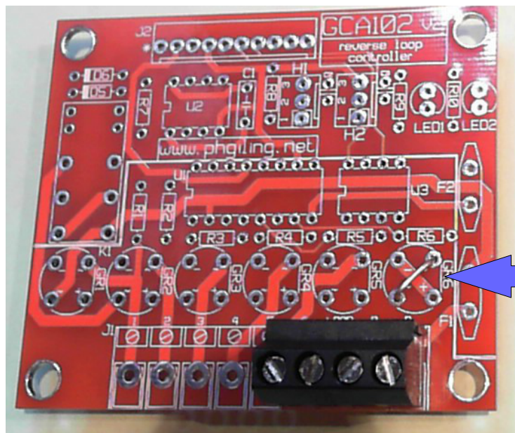
Wire bridge
